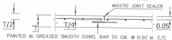
CONSTRUCTION JOINT
