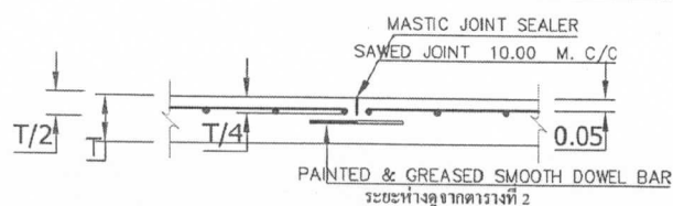
CONTRACTION JOINT
