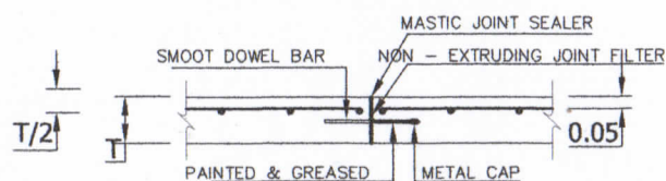
EXPANSION JOINT
