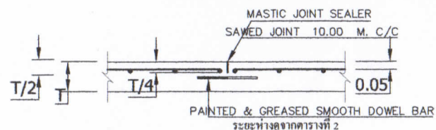
CONTRACTION JOINT
