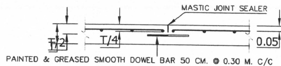
CONSTRUCTION JOINT
