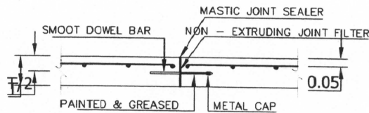
EXPANSION JOINT
