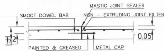
EXPANSION JOINT
