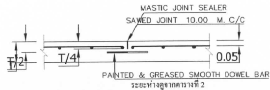
CONTRACTION JOINT
