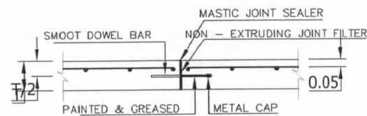
EXPANSION JOINT
