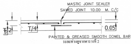
CONTRACTION JOINT
